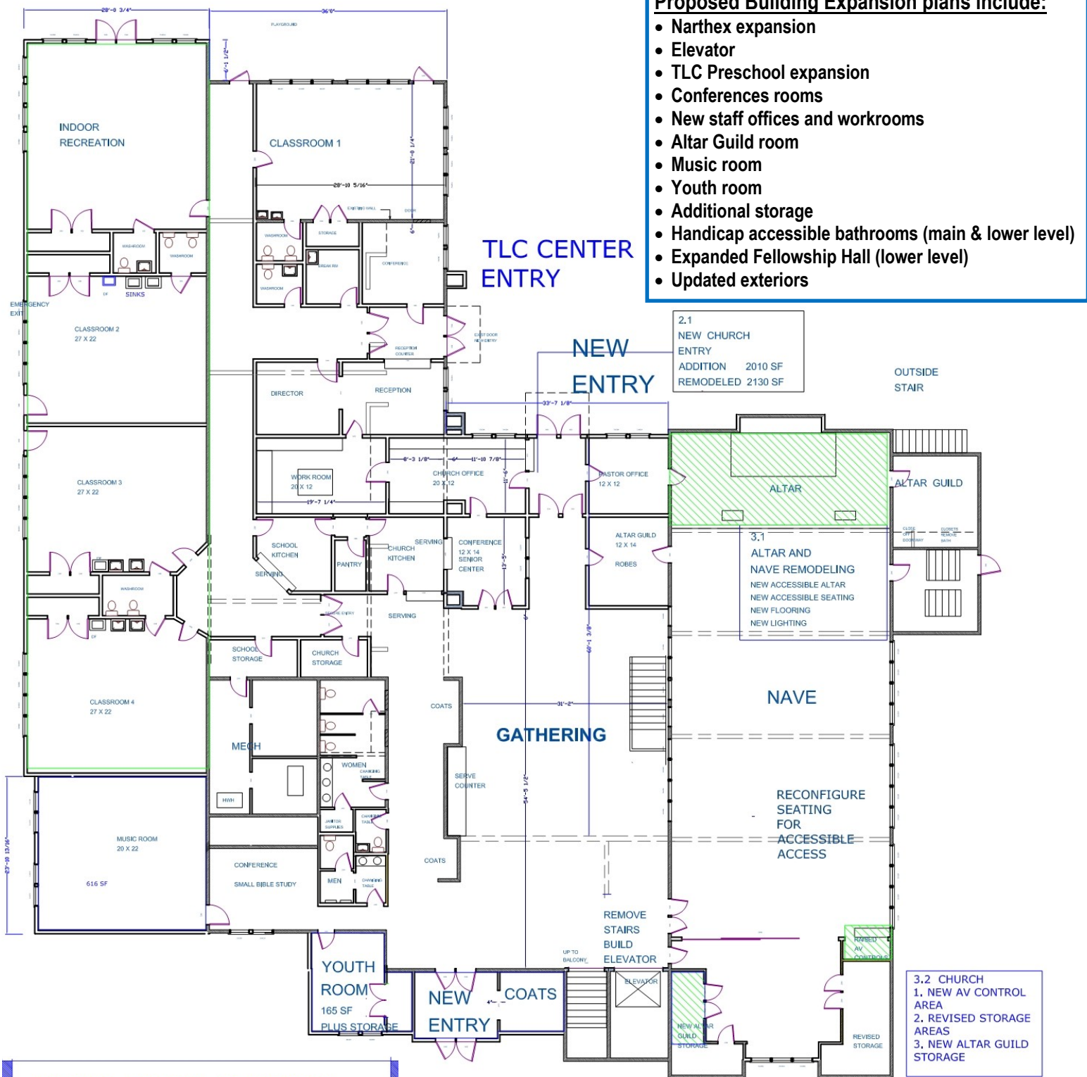
Proposed Expansion — First Floor Plan
